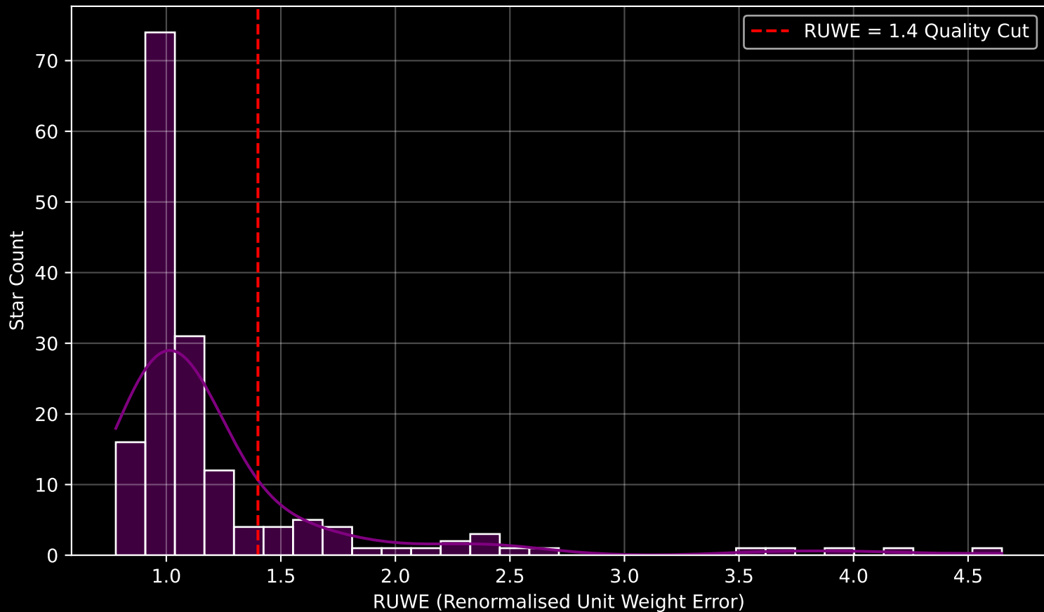
GAPOGEE DR17 Field [200+34_MGA] RUWE Distribution (n= 165)
