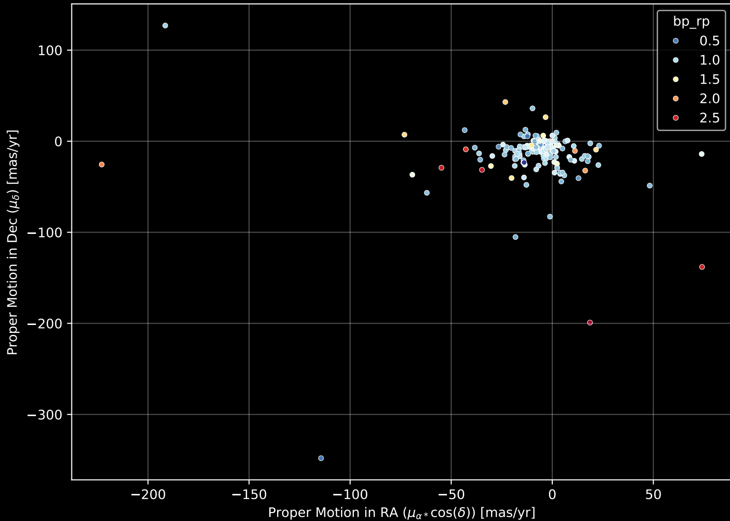
APOGEE DR17 Field: [200+34_MGA] Proper Motion Diagram (n= 173)
