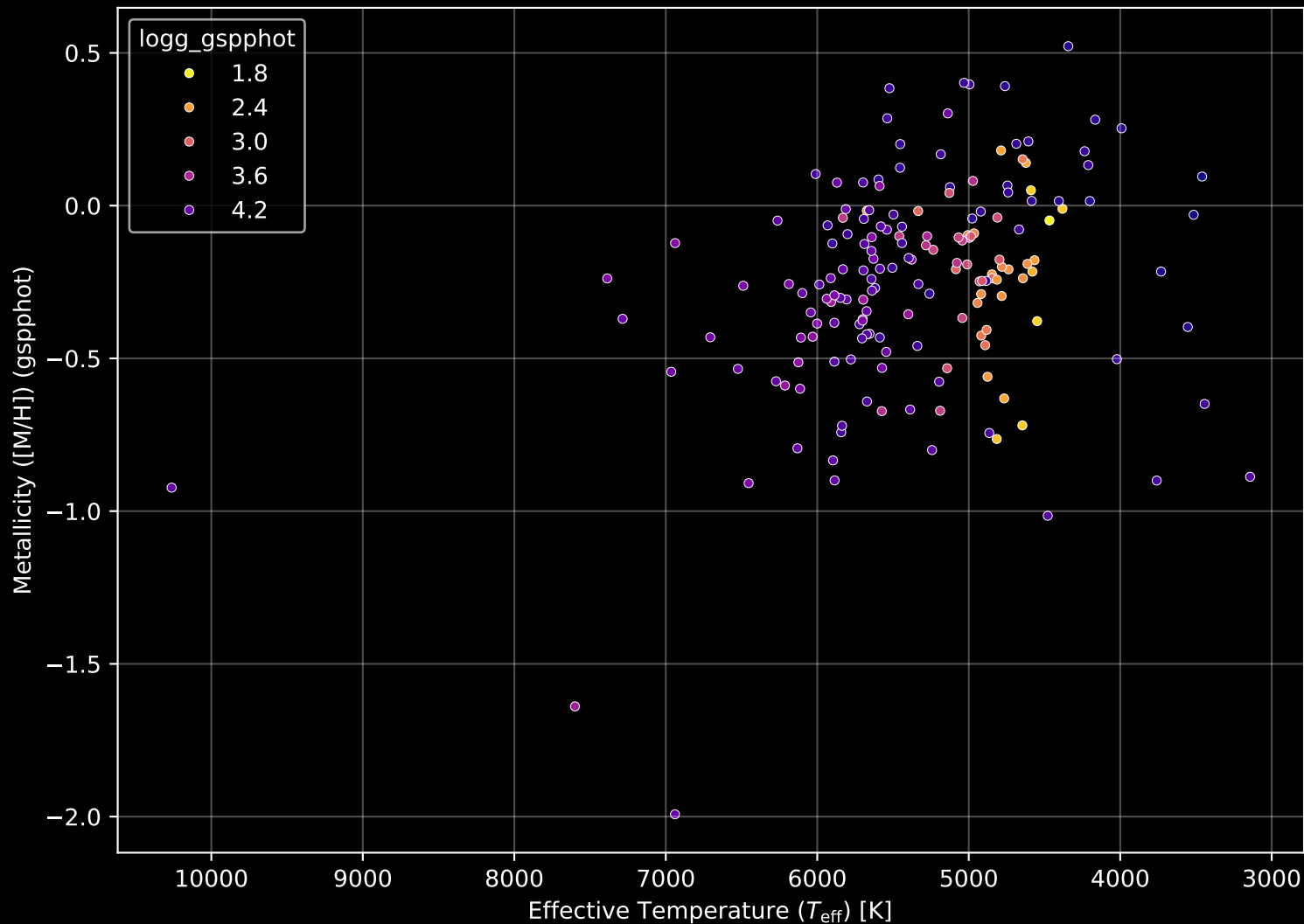
APOGEE DR17 Field: [200+34_MGA] Stellar Population Parameters (n= 173)
