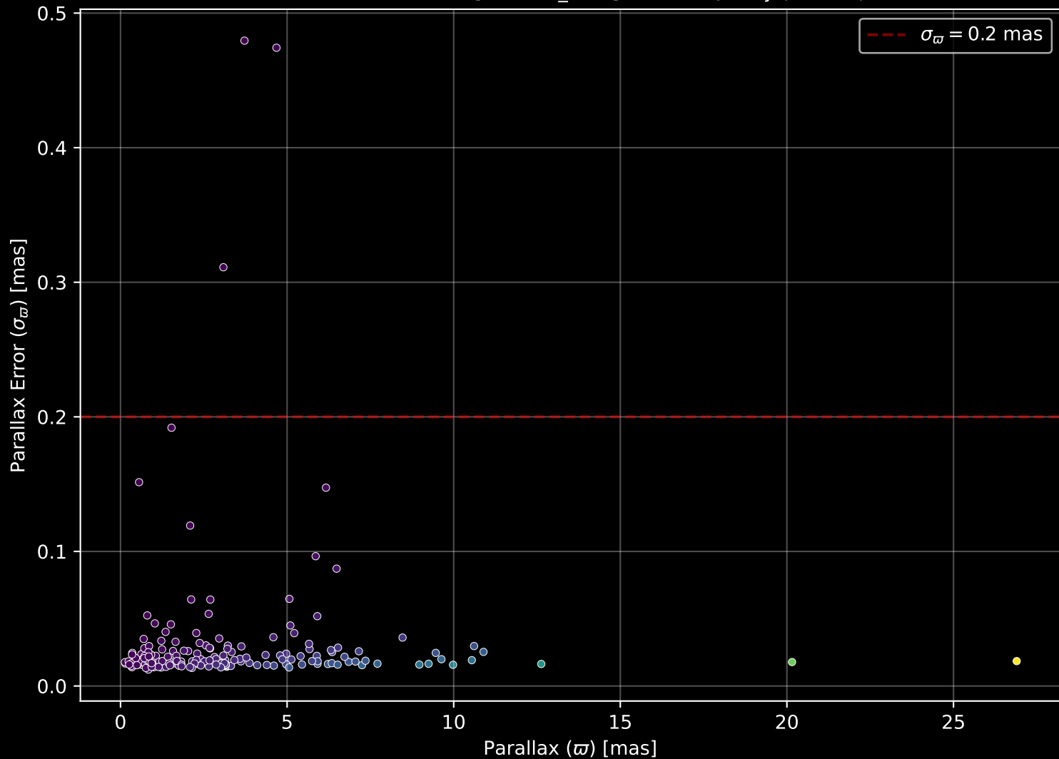
APOGEE DR17 Field: [200+34_MGA] Parallax Quality (n= 173)
