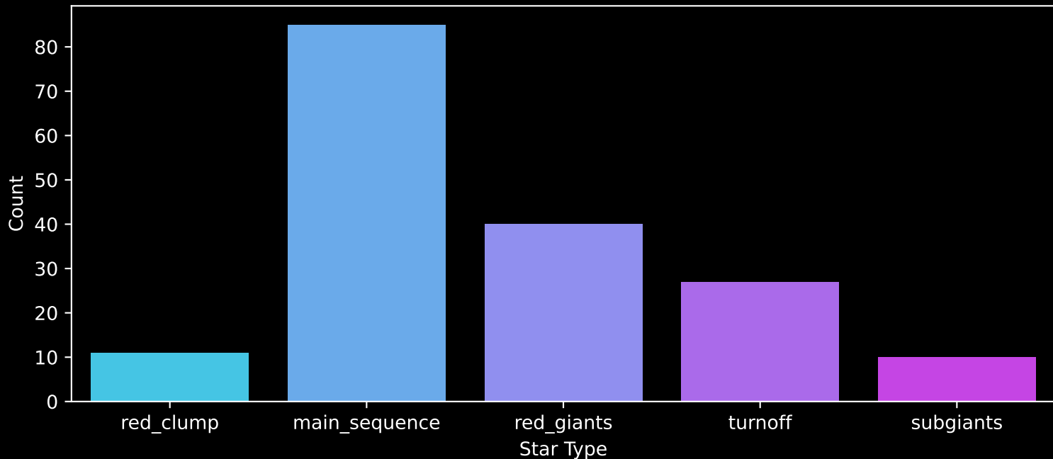
APOGEE DR17 Field: [200+34_MGA] Count plot of Star Type
